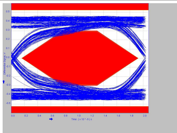
Figure 8-20. 4 Meter Post-Channel Without TUSB216I
