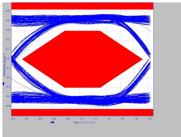
Figure 8-19. 2 Meter Post-Channel With TUSB216I BOOST=1 RX_SEN=HIGH
