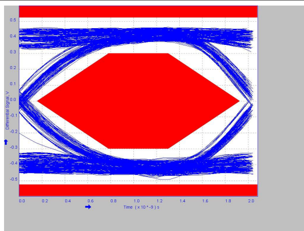
Figure 8-21. 4 Meter Post-Channel With TUSB216I BOOST=2 RX_SEN=MED
