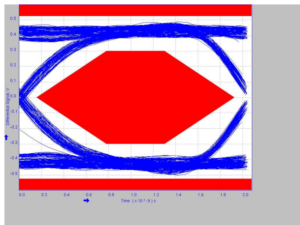
Figure 8-16. 1 Meter Post-Channel With TUSB216I BOOST=0 RX_SEN=HIGH
