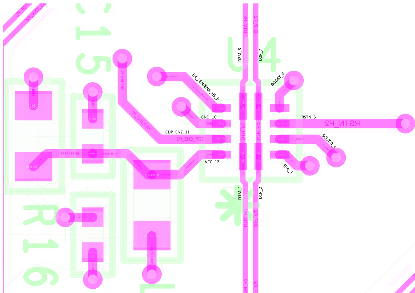
Figure 10-1. Layout Example
