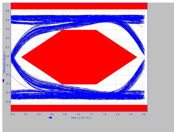
Figure 8-17. 2 Meter Post-Channel Without TUSB216I
