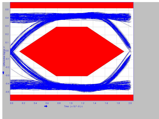
Figure 8-18. 2 Meter Post-Channel With TUSB216I BOOST=1 RX_SEN=MED
