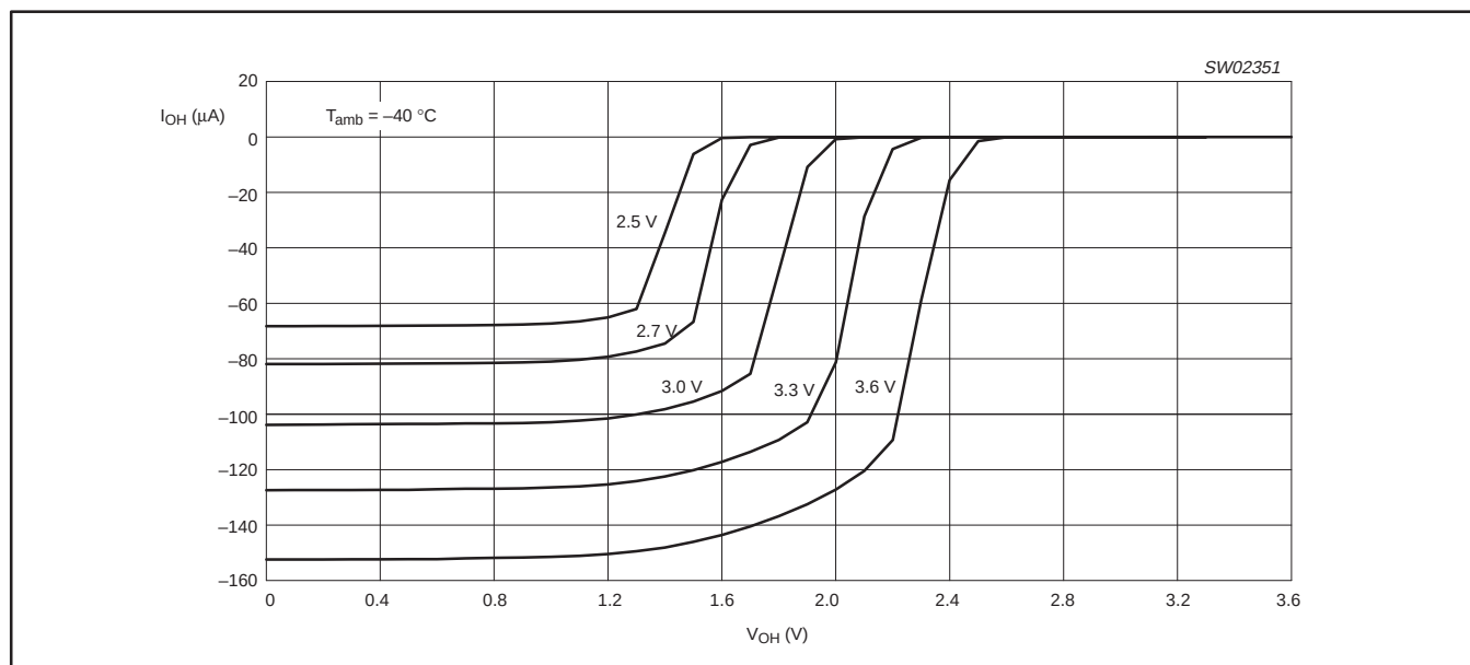
Figure 22. V_{OH} versus I_{OH} ( T_{amb} = -40\text{ °C} )
