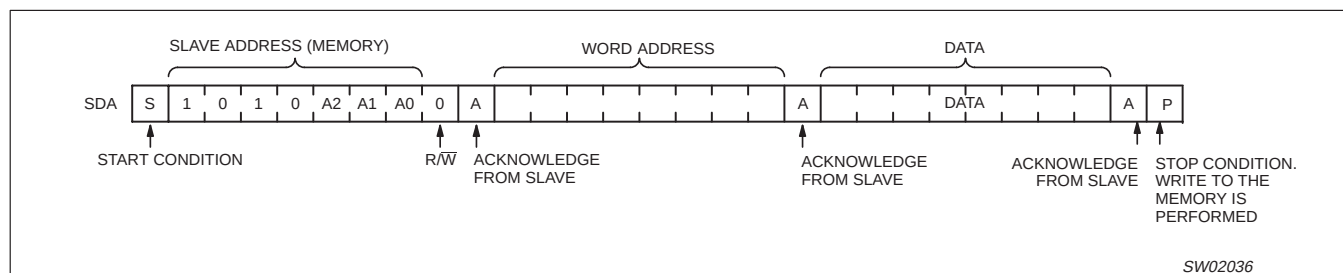
Figure 9. Byte write
