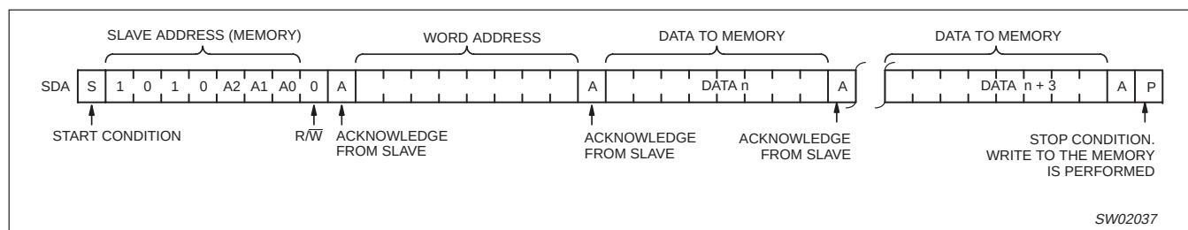
Figure 10. Page Write
