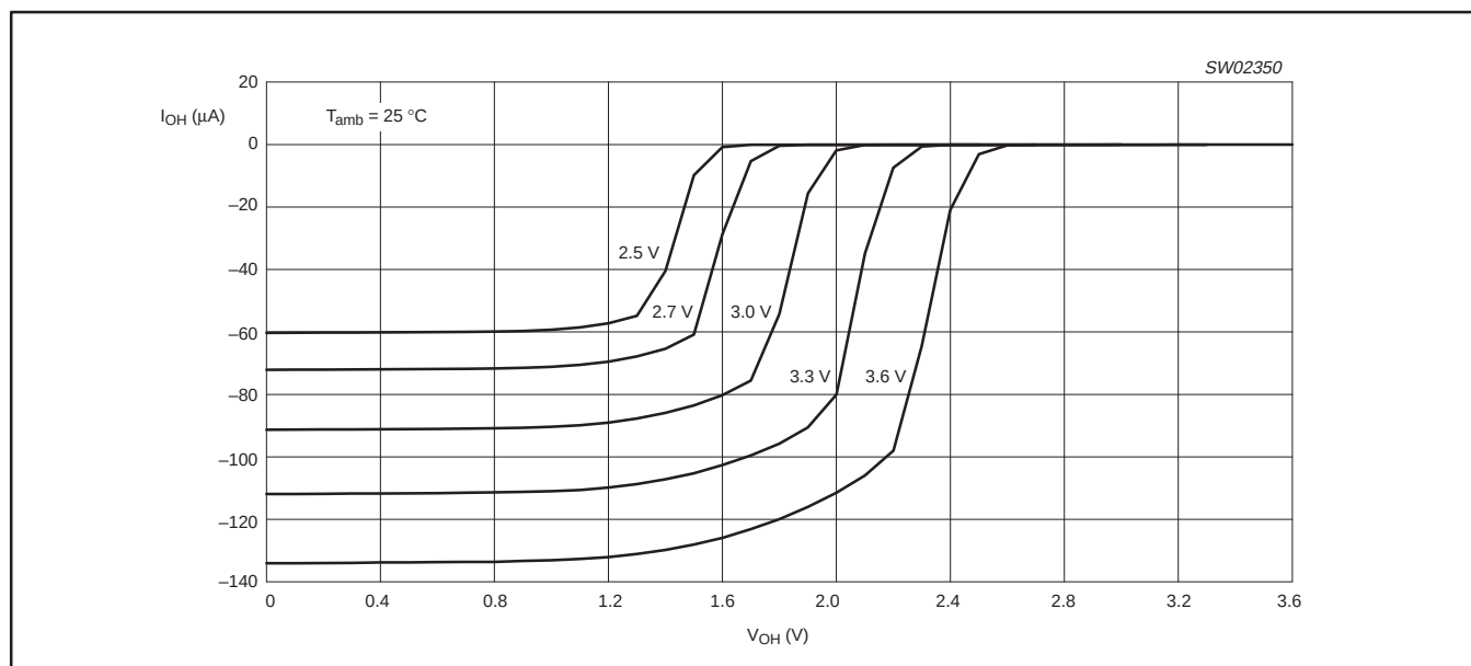
Figure 23. V_{OH} versus I_{OH} ( T_{amb} = 25\text{ °C} )
