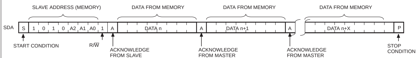
Figure 13. Sequential Read
