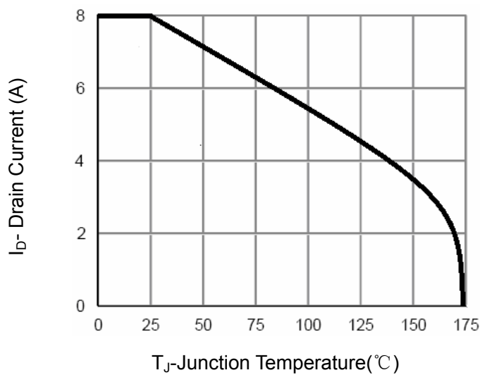
Figure 11 Current De-rating
