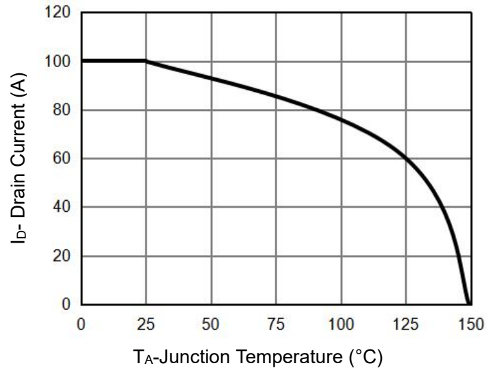
Figure 10 Current De-rating
