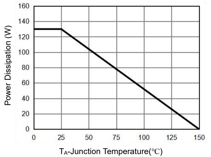
Figure 9 Power De-rating
