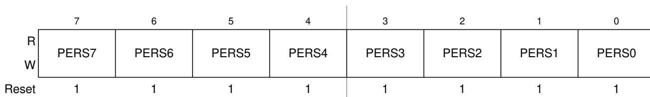
Figure 24-25. Port S Pull Device Enable Register (PERS)
