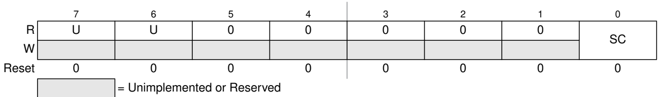
Figure 5-11. ATD Test Register 1 (ATDTEST1)
