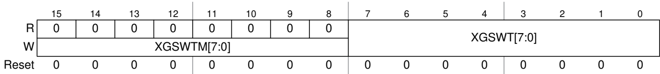
Figure 6-7. XGATE Software Trigger Register (XGSWT)
