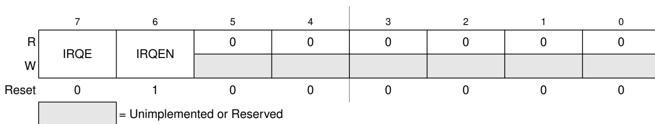
Figure 24-12. IRQ Control Register (IRQCR)
