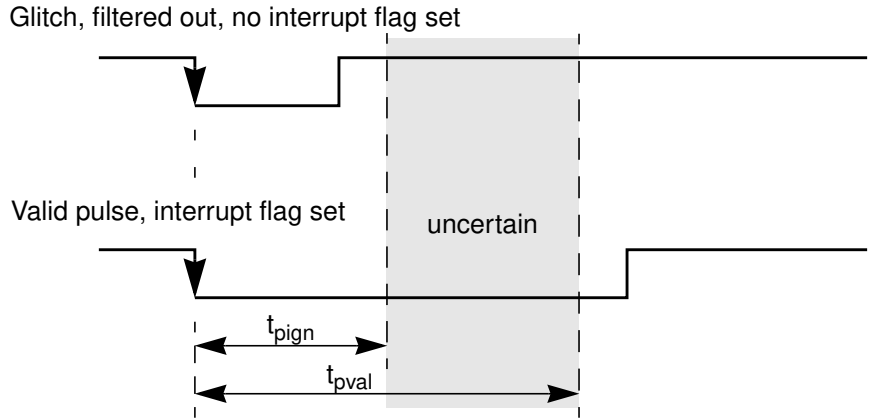
Figure 24-69. Interrupt Glitch Filter on Port P, H, and J (PPS = 0)
