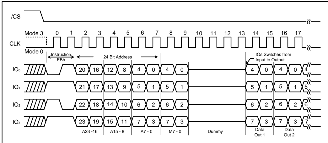
Figure 17d. Fast Read Quad I/O Instruction (Initial instruction or previous M7-0 ≠ Axxh, QPI mode, 108MHz)
