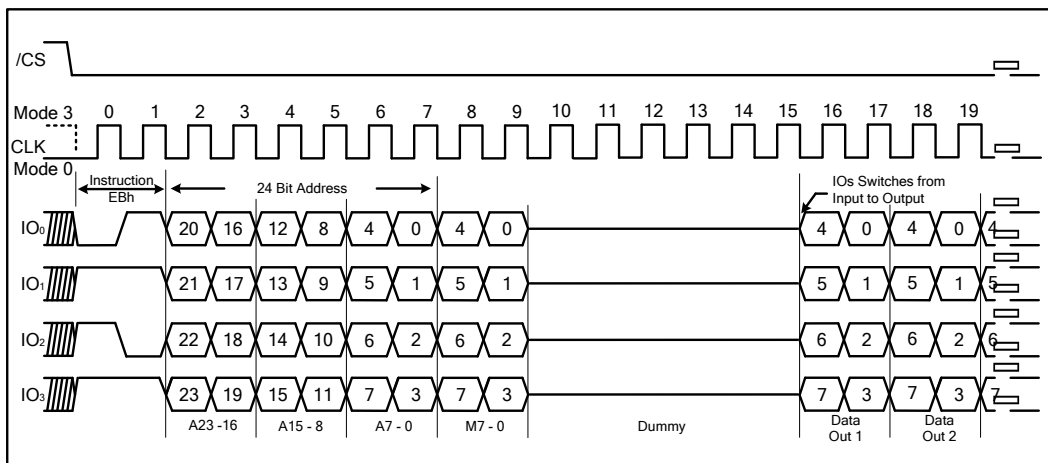
Figure 17e. Fast Read Quad I/O Instruction (Initial instruction or previous M7-0 ≠ Axxh, QPI mode, 133MHz)
