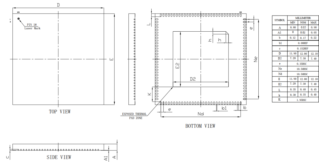
Package Dimensions (QFN124)
