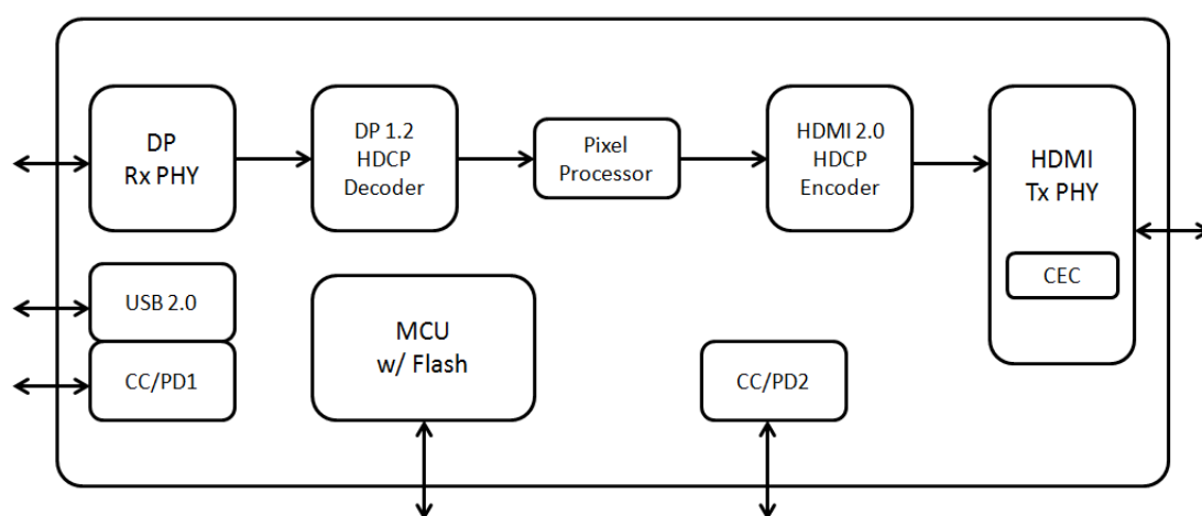
Figure 1. Top Diagram
