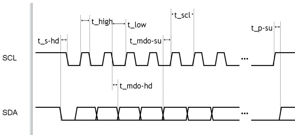
(a) I2C master data out
