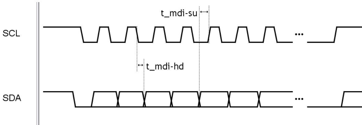
(b) I2C master data in
