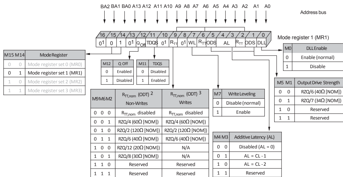
Figure 42 : Mode Register 1 (MR1) Definition
