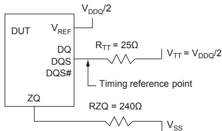
Figure 18 : Reference Output Load for AC Timing and Output Slew Rate
