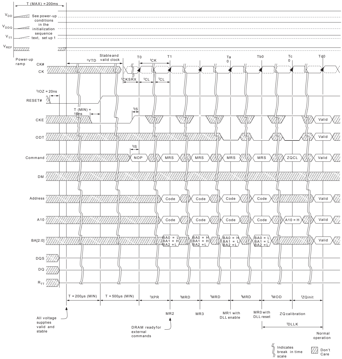
Figure 37 : Initialization Sequence
