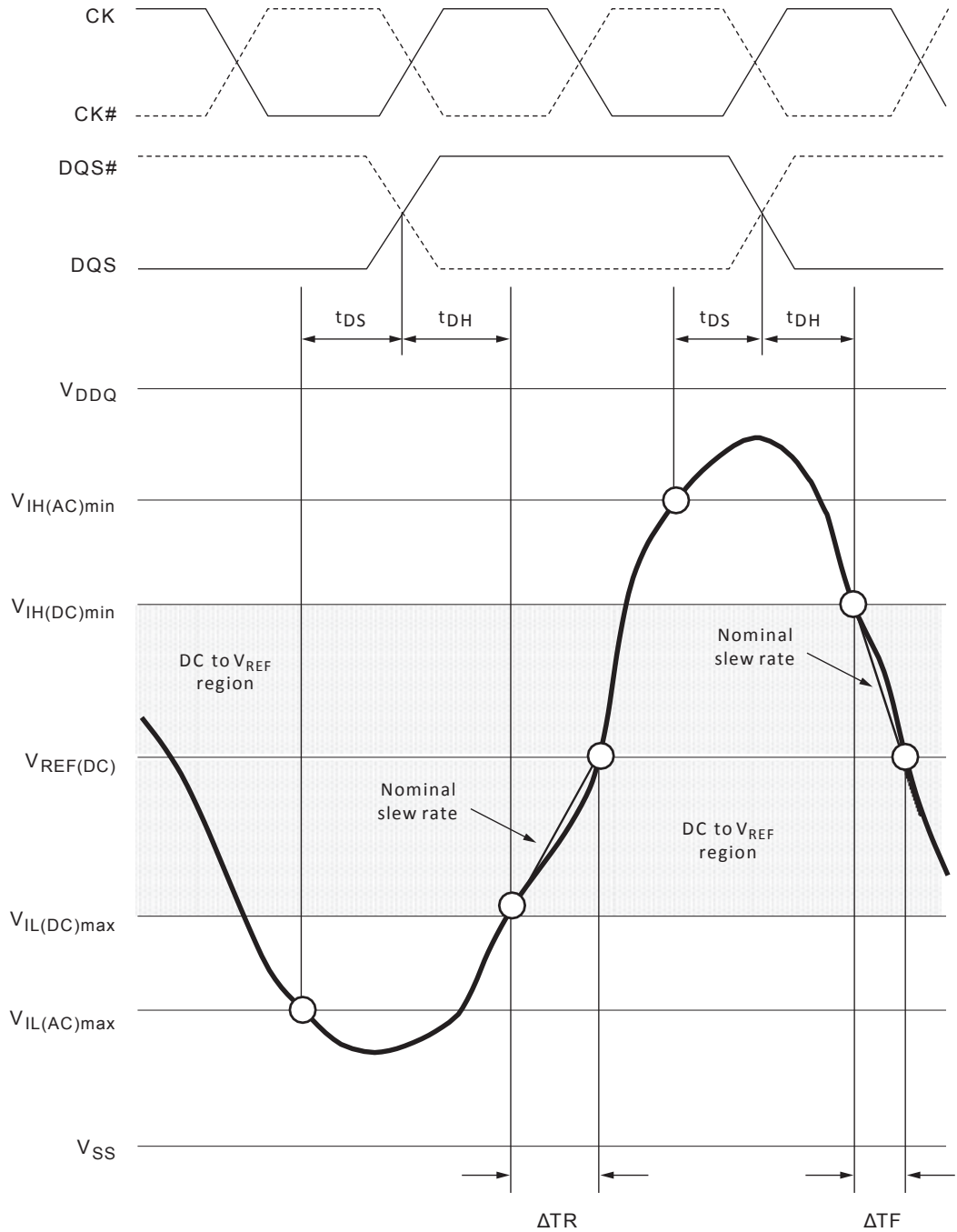
Figure 26 : Nominal Slew Rate for tDH (DQ – Strobe)
