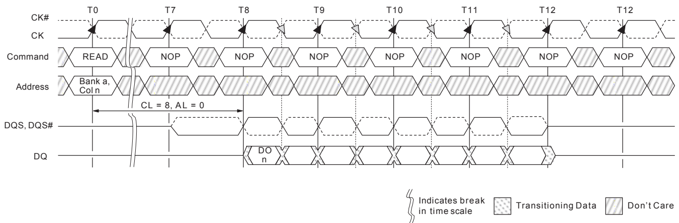
Figure 55 : READ Latency
