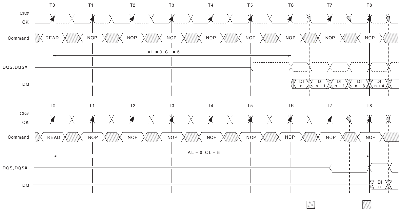
Figure 41 : READ Latency
