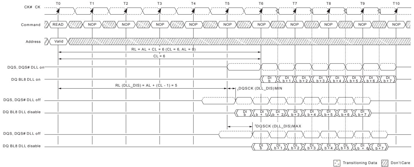
Figure 32 : DLL Disable tDQSK
