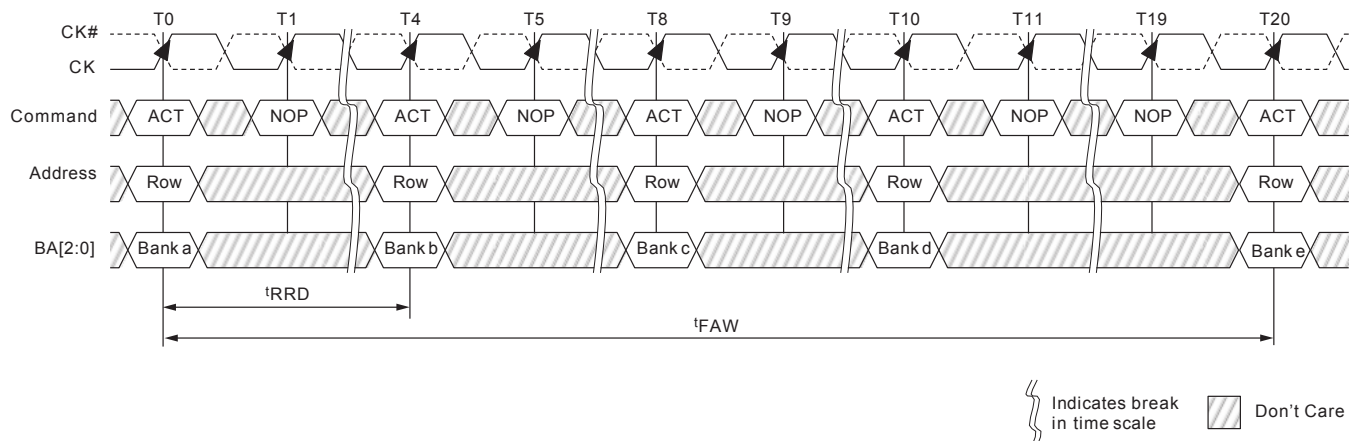
Figure 54 : Example: tFAW
