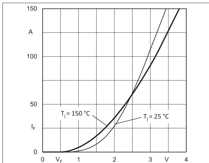
Fig. 10: Typ. CAL diode forward characteristic
