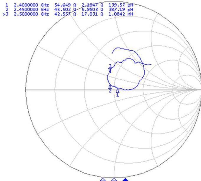
▶ S22 Smith (R+jX) Scale 1.000U
