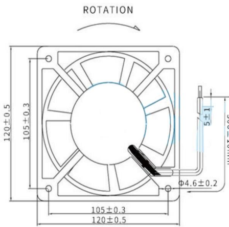
DIMENSIONS DRAWING(unit:mm)
