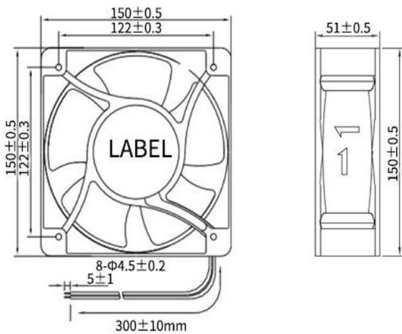
DIMENSIONS DRAWING(unit:mm)
