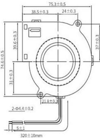
DIMENSIONS DRAWING(unit:mm)
