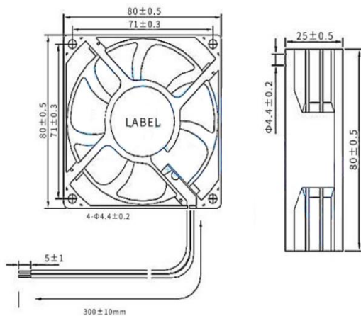
DIMENSIONS DRAWING(unit:mm)
