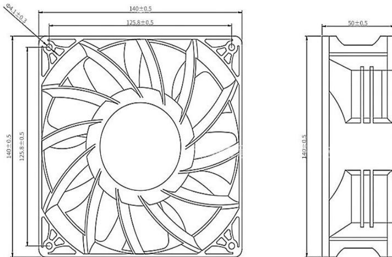
DIMENSIONS DRAWING(unit:mm)
