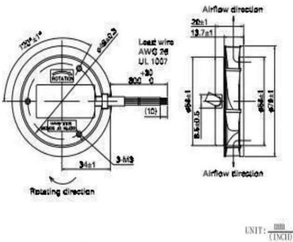
DIMENSIONS DRAWING(unit:mm)
