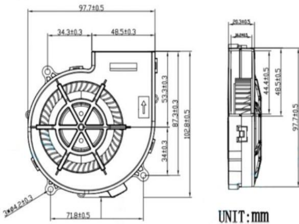
DIMENSIONS DRAWING(unit:mm)
