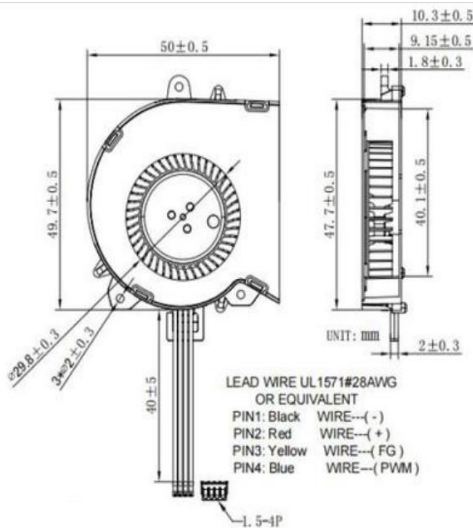
DIMENSIONS DRAWING(unit:mm)
