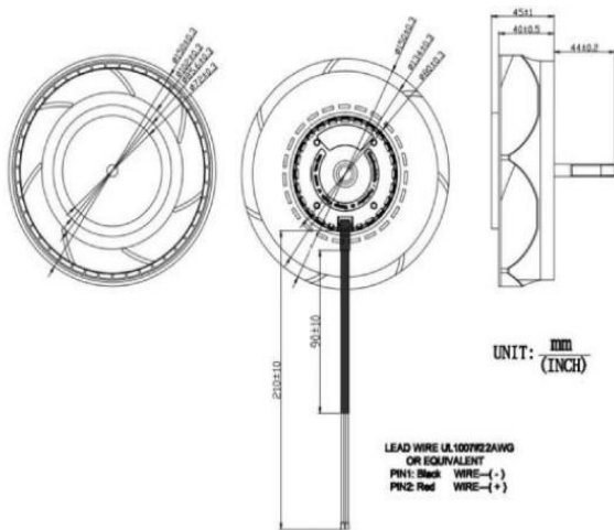
DIMENSIONS DRAWING(unit:mm)
