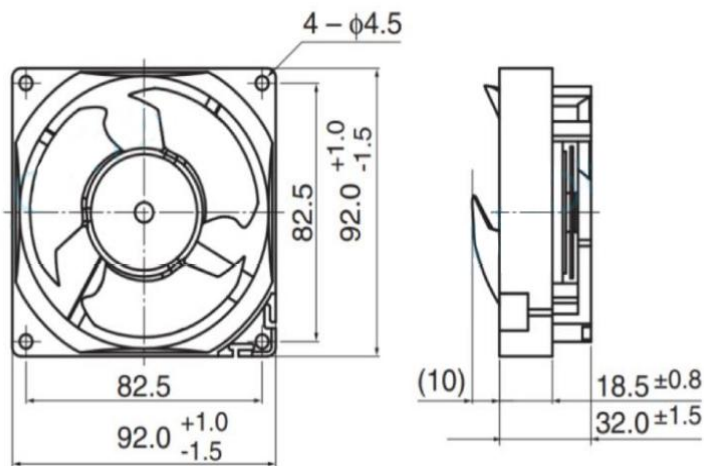
DIMENSIONS DRAWING(unit:mm)
