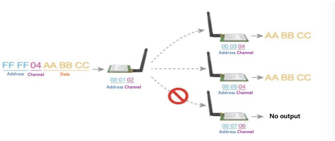
Figure 5-2 Broadcasting Transmission
