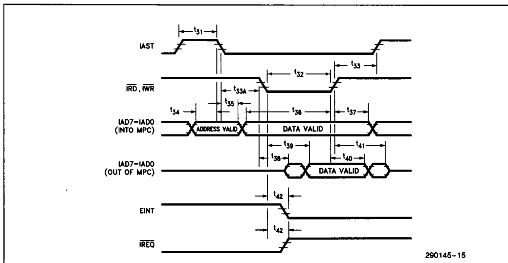
Figure 7-4. Interconnect Bus Timing
