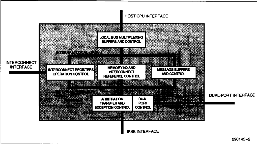
Figure 3-1. MPC Bus Interfaces
