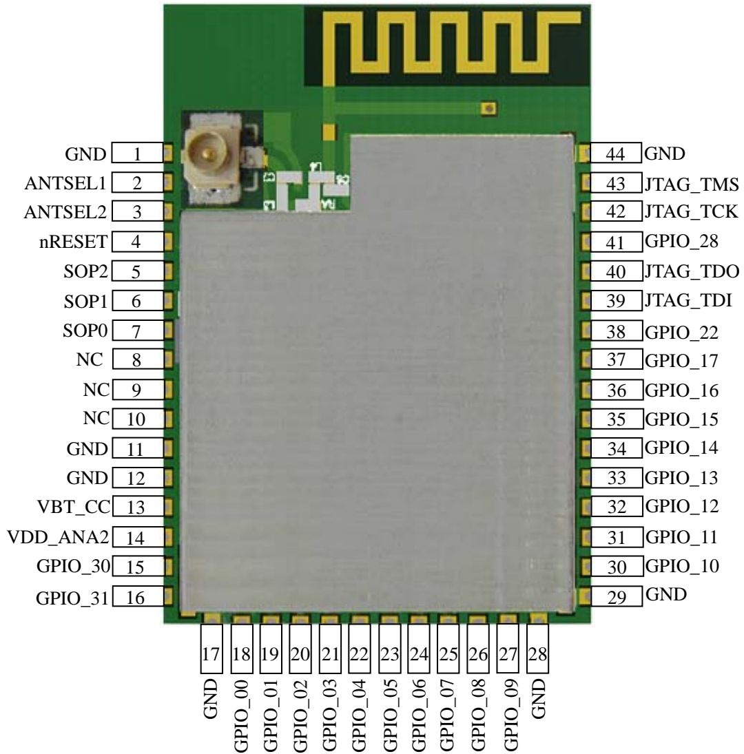
Figure 2-1. TA3200R1D Pin Diagram
