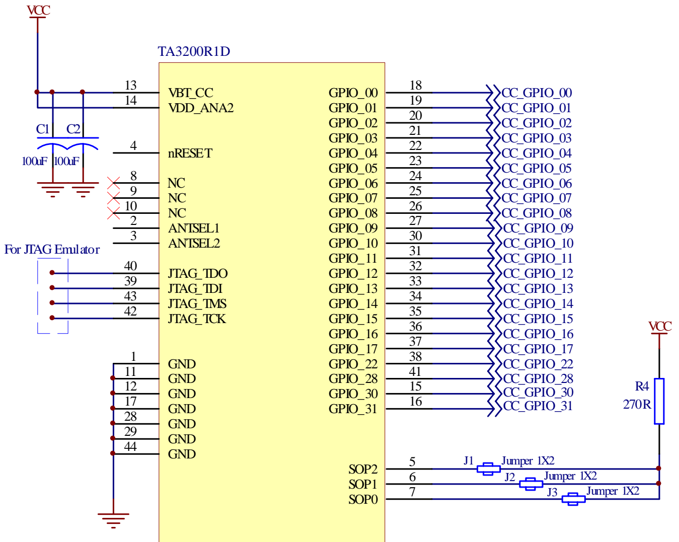
Figure 4-1. TA3200R1D Module Reference Schematic
