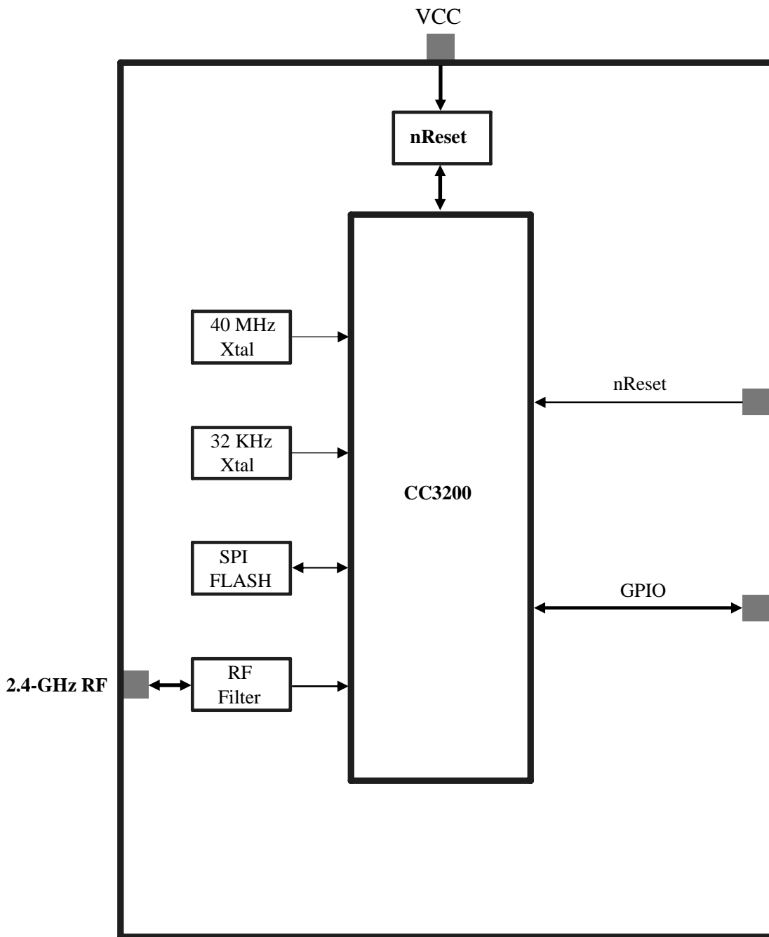
Figure 1-1. TA3200R1D Module Functional Block Diagram
