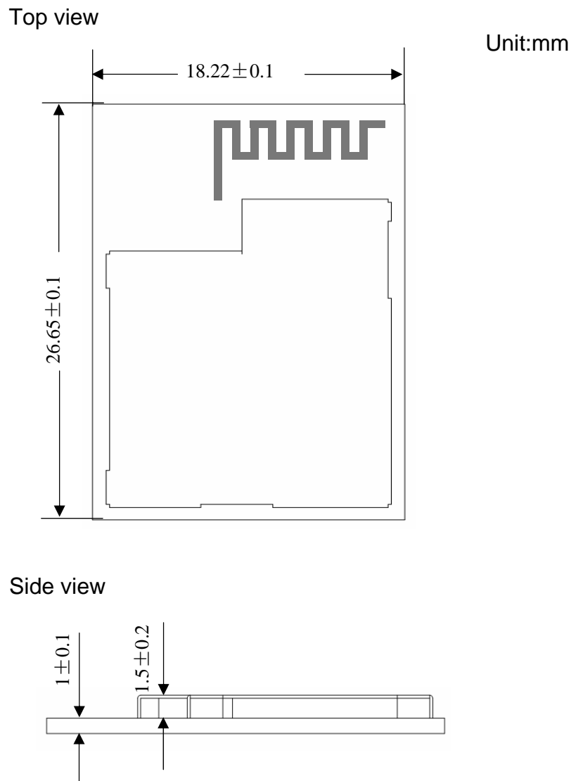
Figure 5-1. Mechanical Drawing
