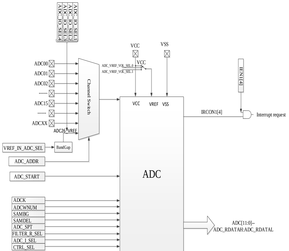
ADC structure block diagram
