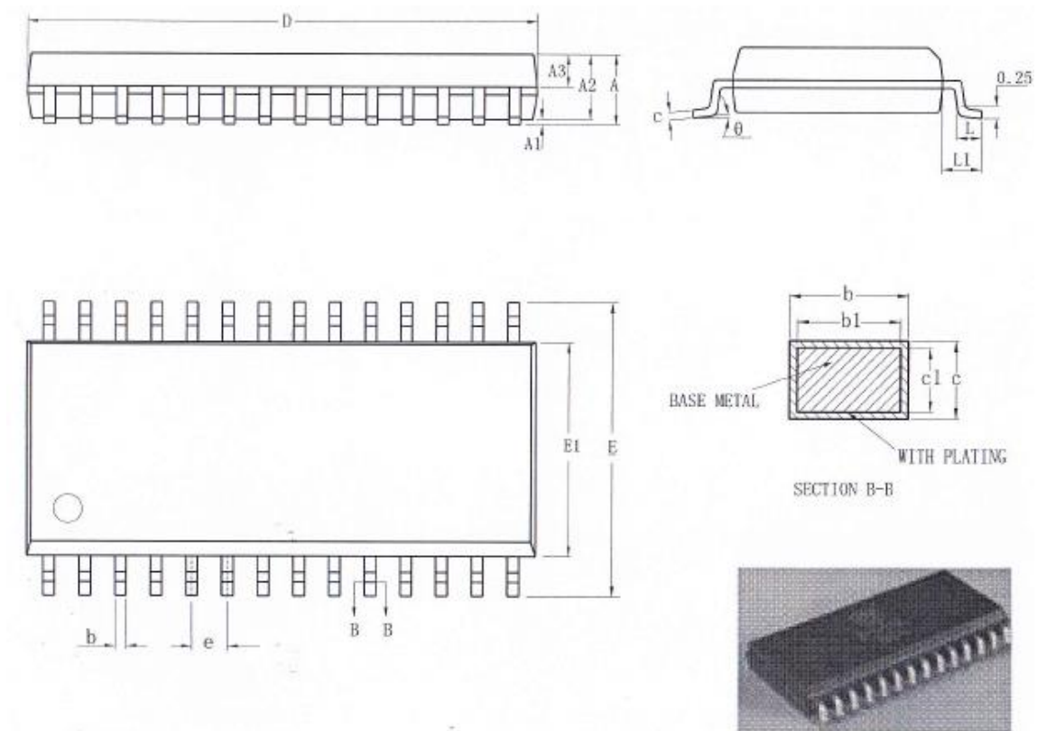
SOP28 package
