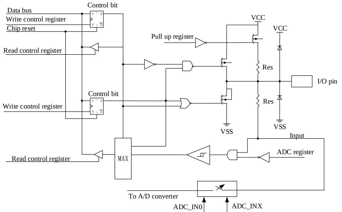
ADC IO structure
