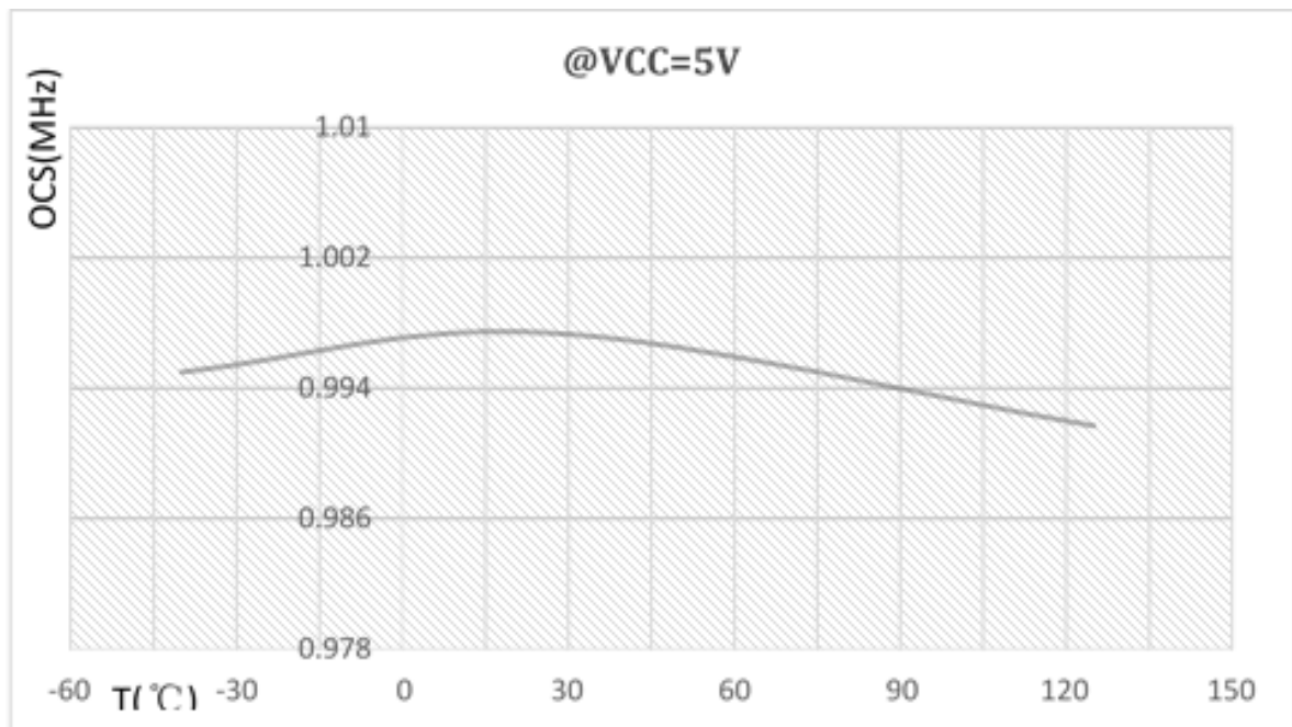
RC1M (OSC) temperature characteristic curve
