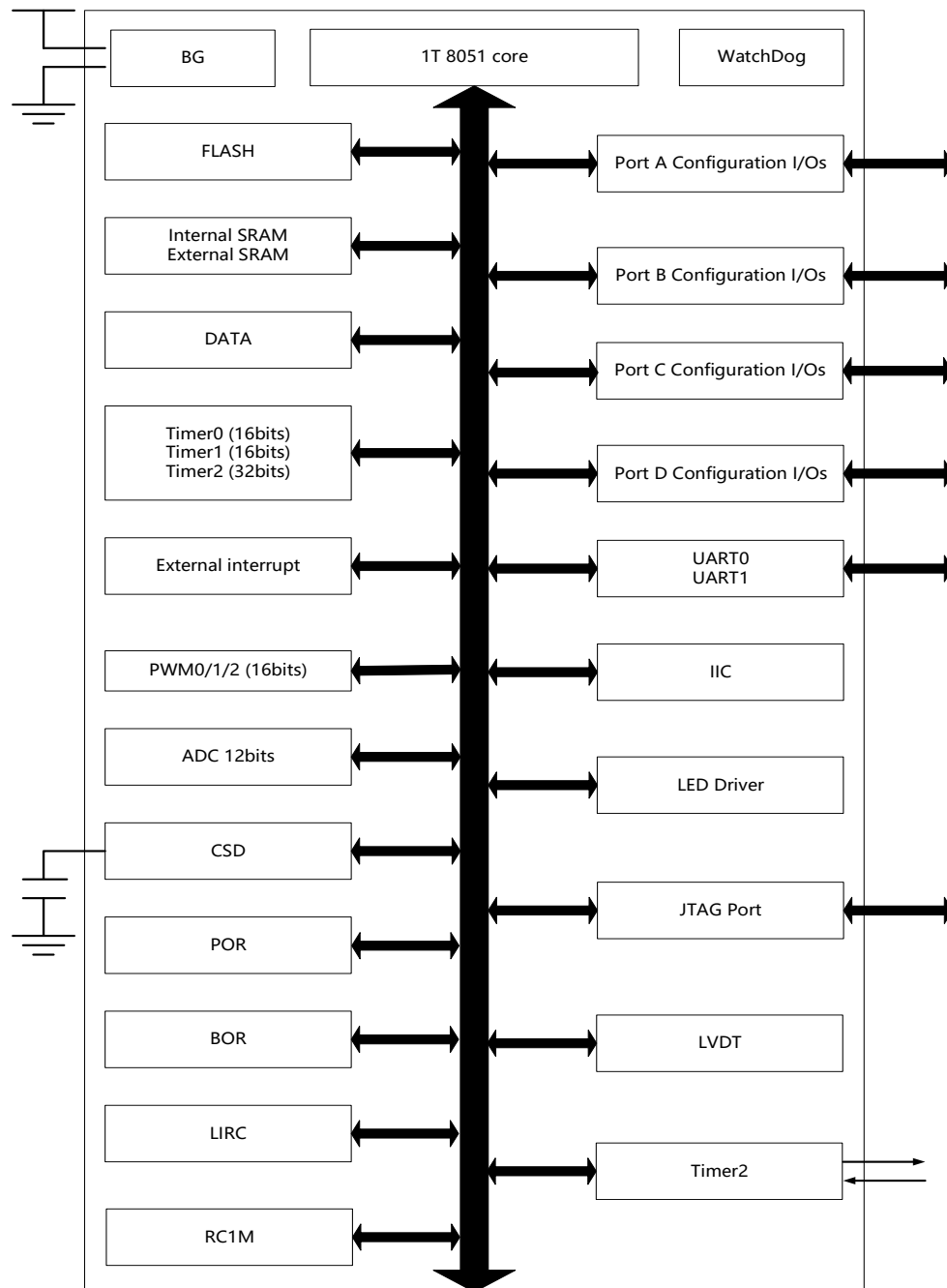
System architecture
