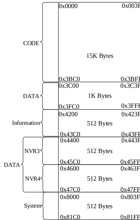
Flash Storage Architecture
