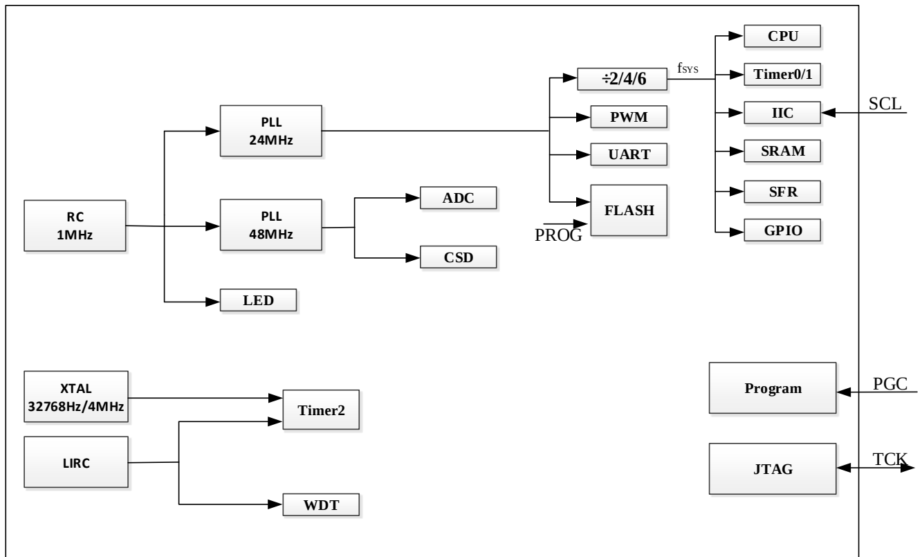
Clock diagram
