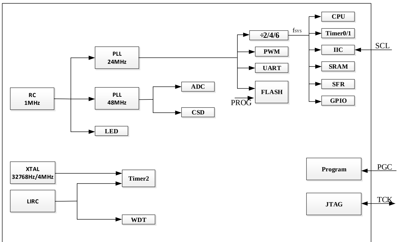
Clock block diagram
