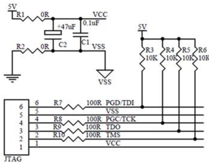
JTAG circuit connection
