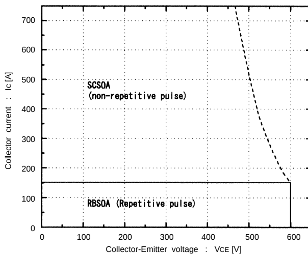
Reversed biased safe operating area +V_{GE}=15V , -V_{GE} \leq 15V , T_J \leq 125^\circ C , R_G \geq 33\text{ ohm}
