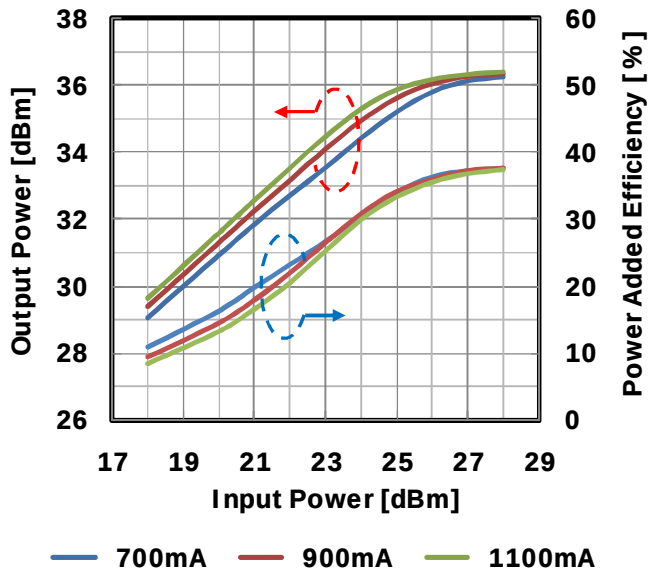
Input Power vs. Output Power, Power Added Efficiency by Quiescent Drain Current V_{DS}=10V @7.9GHz
