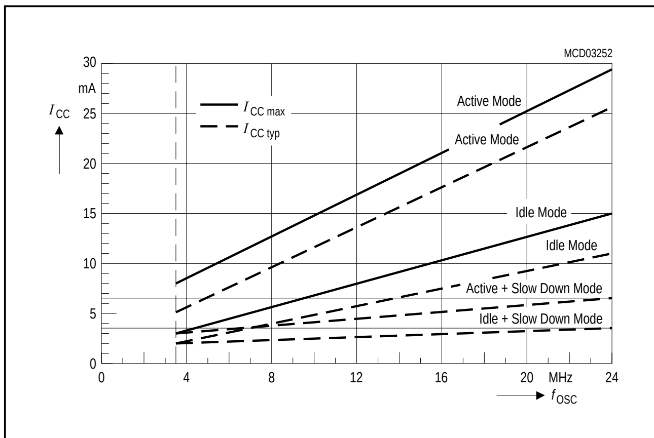
Figure 19 ICC Diagram
