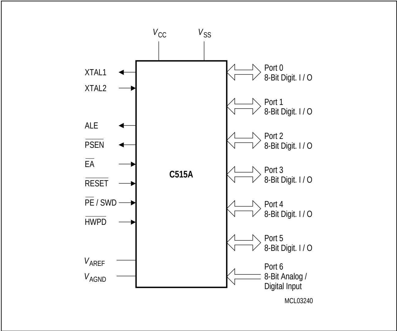
Figure 2 Logic Symbol
