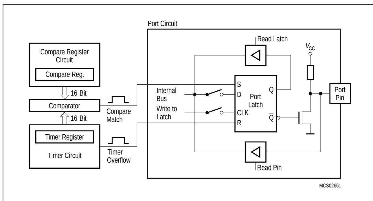
Figure 11 Port Latch in Compare Mode 0
