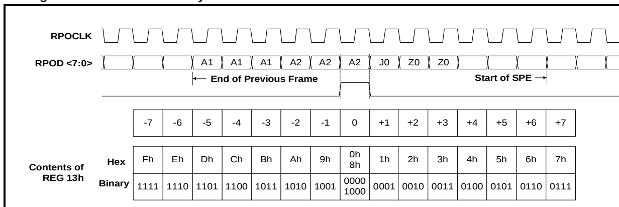
Figure 5. Receive Frame Synchronization and Frame Pulse Position
