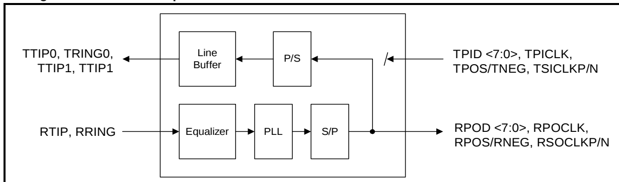
Figure 14. Remote Loopback
