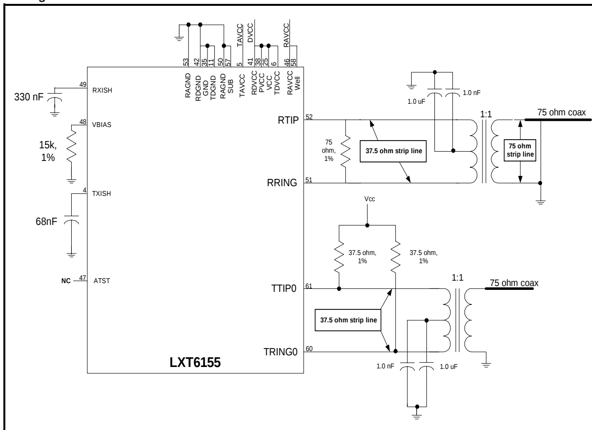
Figure 17. 75 \Omega Coax Cable Interface
