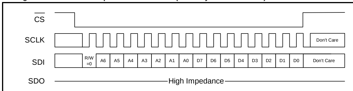
Figure 10. Serial Data Input Word Structure (Write Cycle: \overline{R/W} = Low)
