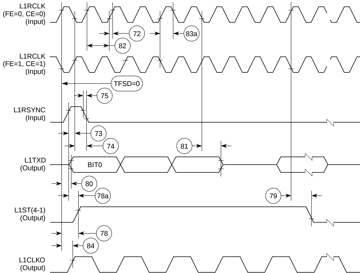
Figure 8-48. SI Transmit Timing with Double Speed Clocking (DSC = 1)
