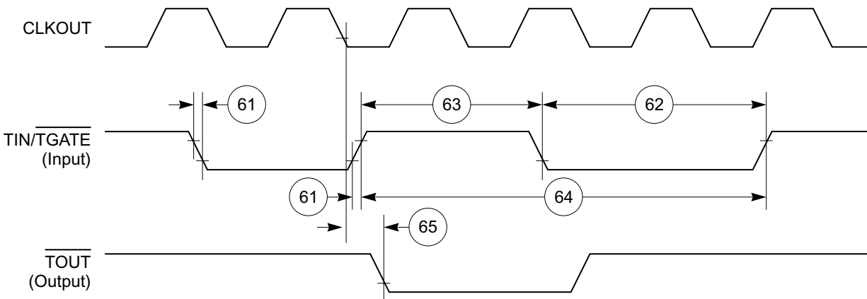
Figure 8-44. CPM General-Purpose Timers Timing Diagram
