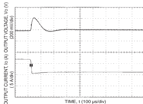
Figure 40. Transient Response to Step Decrease in Load from 50% to 25% of Full Load ( V_i = 48 V_{dc} ).
