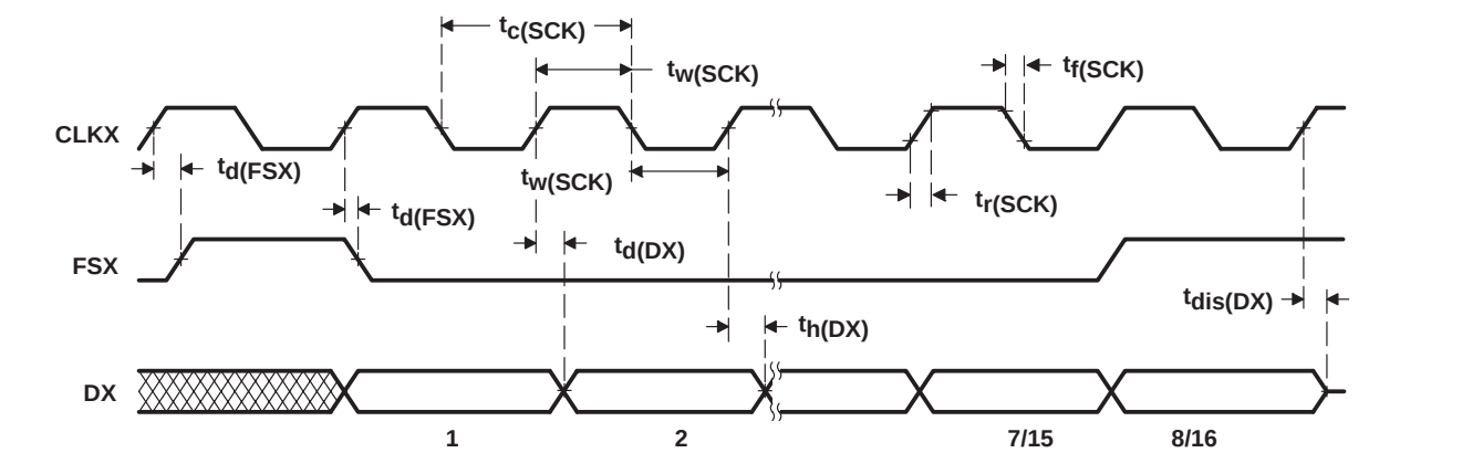
Figure 23. Serial Port Transmit Timing With Internal Clocks and Frames
