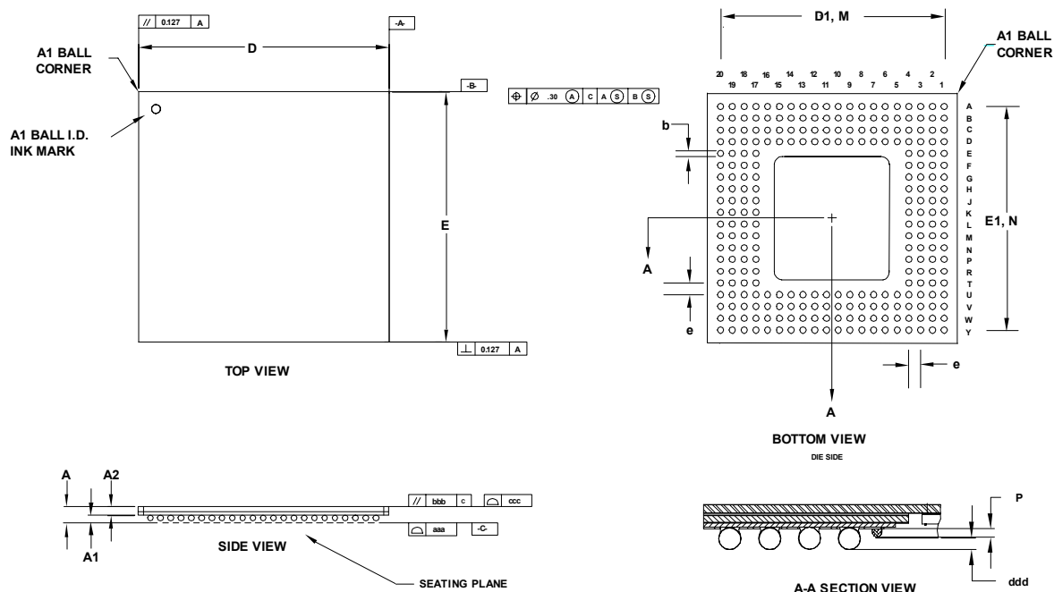
Figure 44 – 256 Pin Enhanced Ball Grid Array (SBGA)
