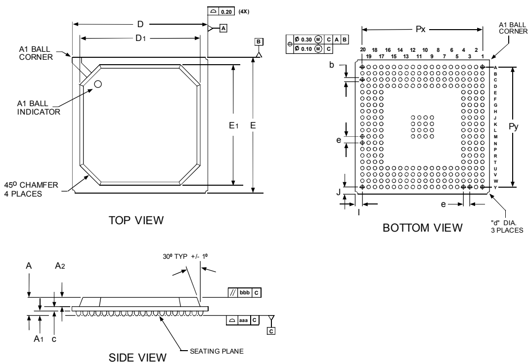
Figure 45 – 272 Pin Plastic Ball Grid Array (PBGA)
