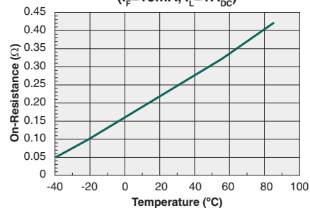
Typical On-Resistance vs. Temperature ( I_F = 10mA , I_L = 1A_{DC} )
