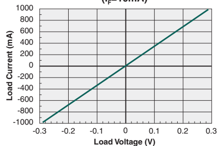
Typical Load Current vs. Load Voltage ( I_F = 10mA )
