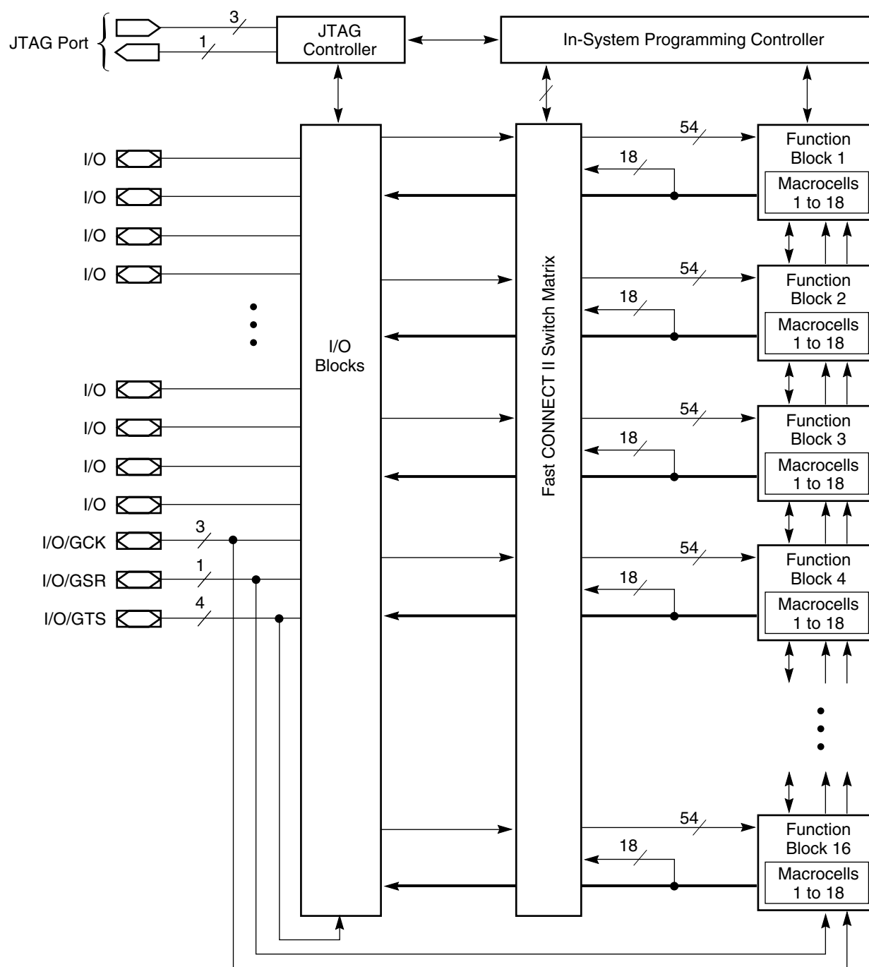
Figure 2: XC95288XL Architecture
