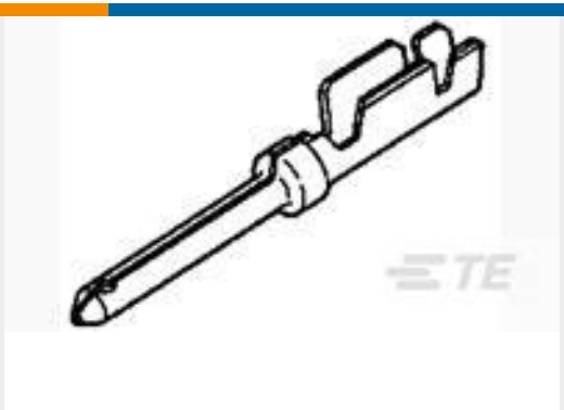
TE Part #1658670-2 PIN CONTACT,22-28 AWG, 22 DF, AMPLIMITE
