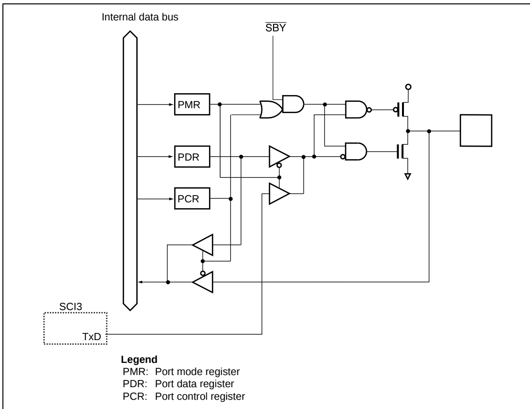
Figure B.5 Port 2 Block Diagram (P22)
