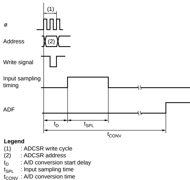
Figure 14.2 A/D Conversion Timing
