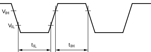
Figure 17.3 Input Timing
