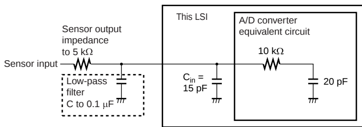
Figure 14.6 Analog Input Circuit Example
