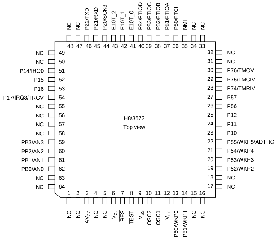
Figure 1.2 Pin Arrangement (FP-64E)
