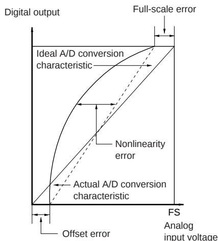
Figure 14.5 A/D Conversion Accuracy Definitions (2)
