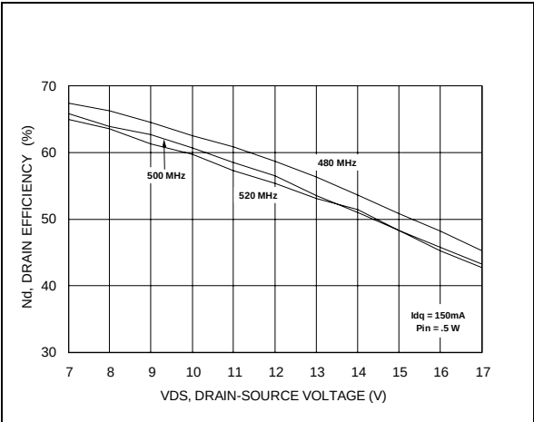
Drain Efficiency vs. Drain Voltage
