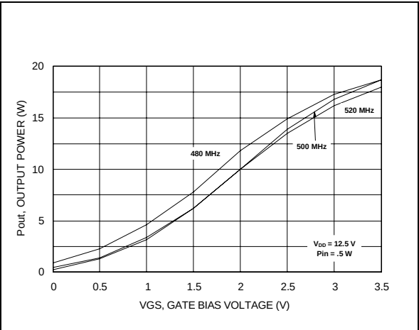
Output Power vs. Gate Bias Voltage
