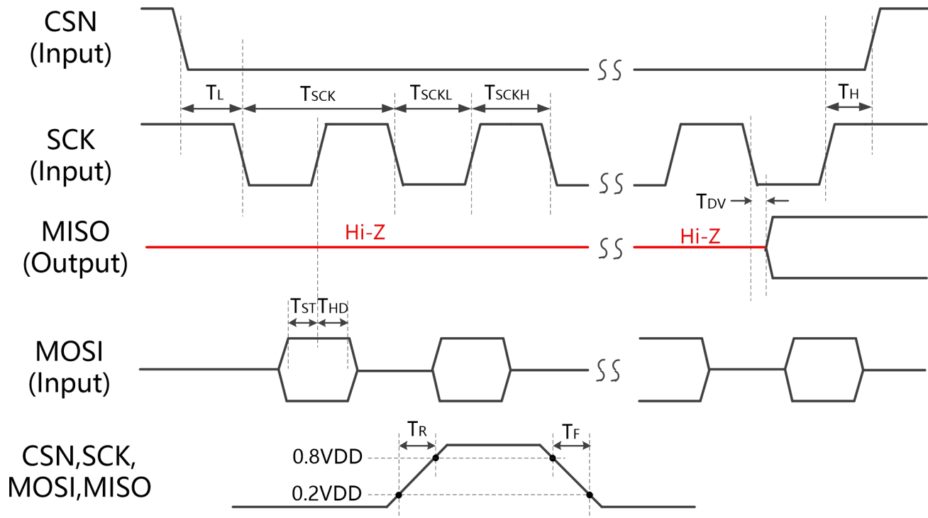
Figure 18: SPI Timing Diagram
