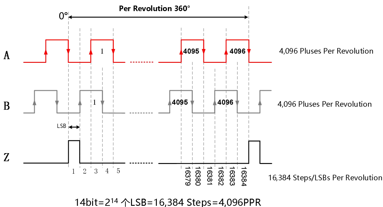
Figure 9: ABZ Output Resolution = 14bit = 4,096PPR
