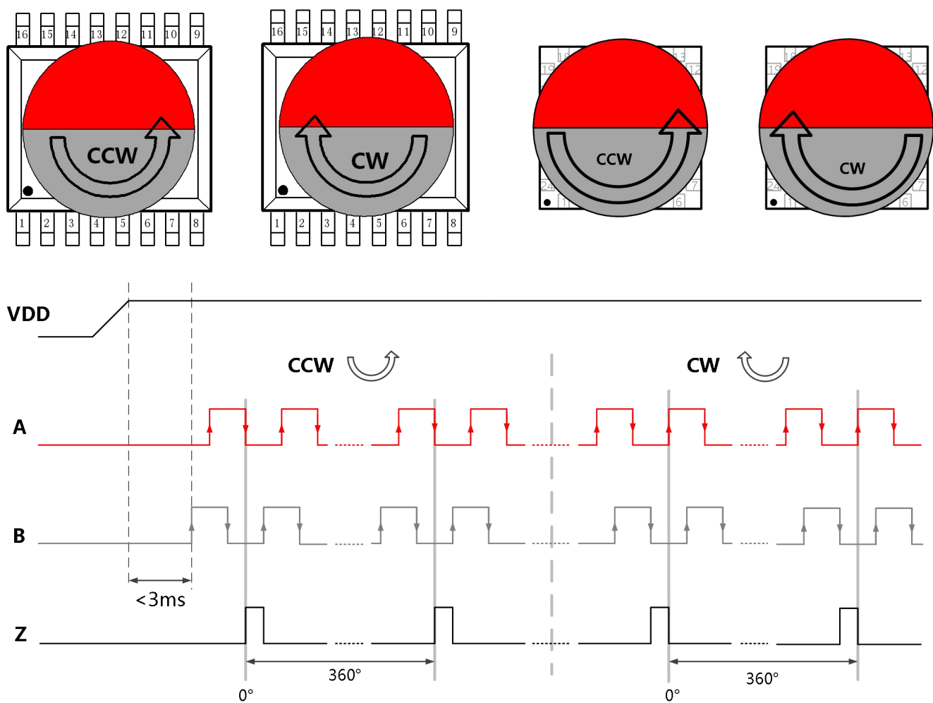
Figure 8: ABZ output with VDD power on
