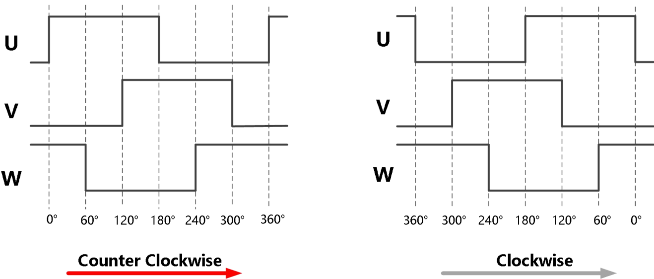
Figure 15: Typical Output Waveform for UVW Mode
