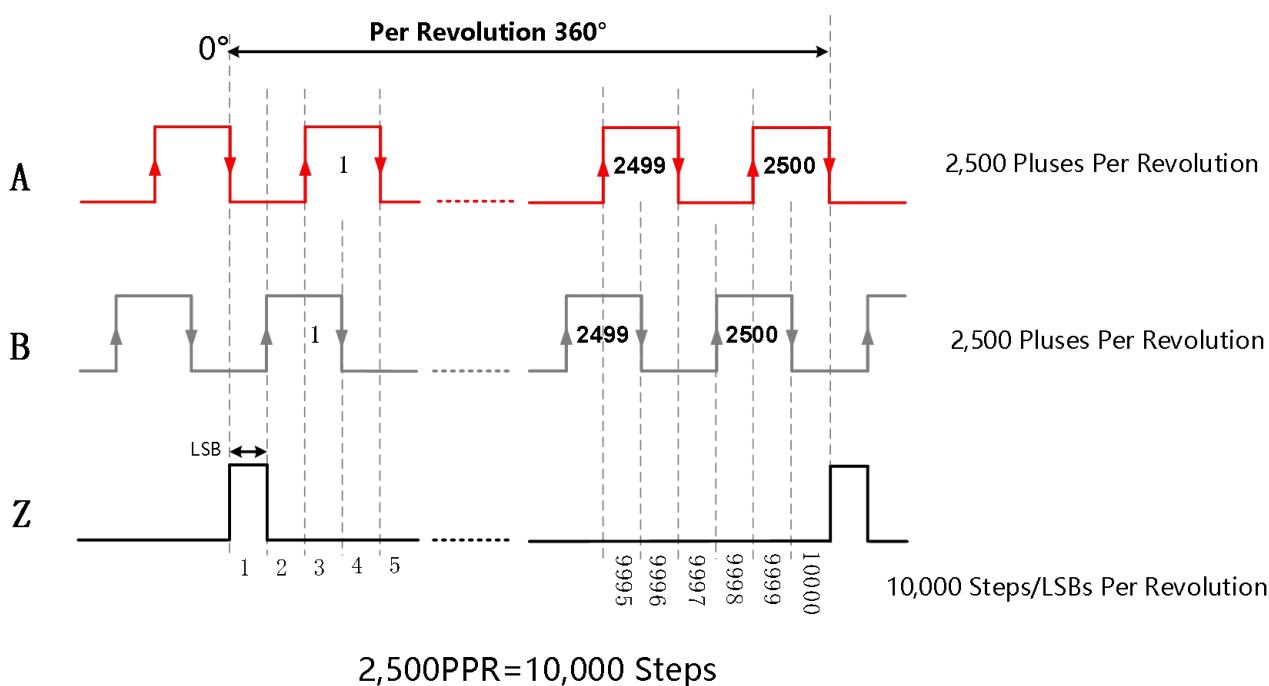
Figure 10: ABZ Output Resolution = 2,500 PPR
