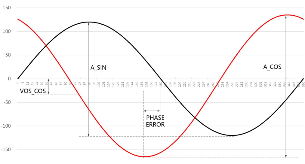
Figure 29: Offset, Gain-Mismatch and Phase-Error
