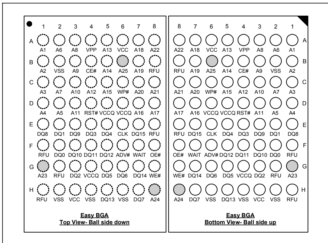
Figure 8. 64-Ball Easy BGA Ballout (64/128/256/512-Mbit)
