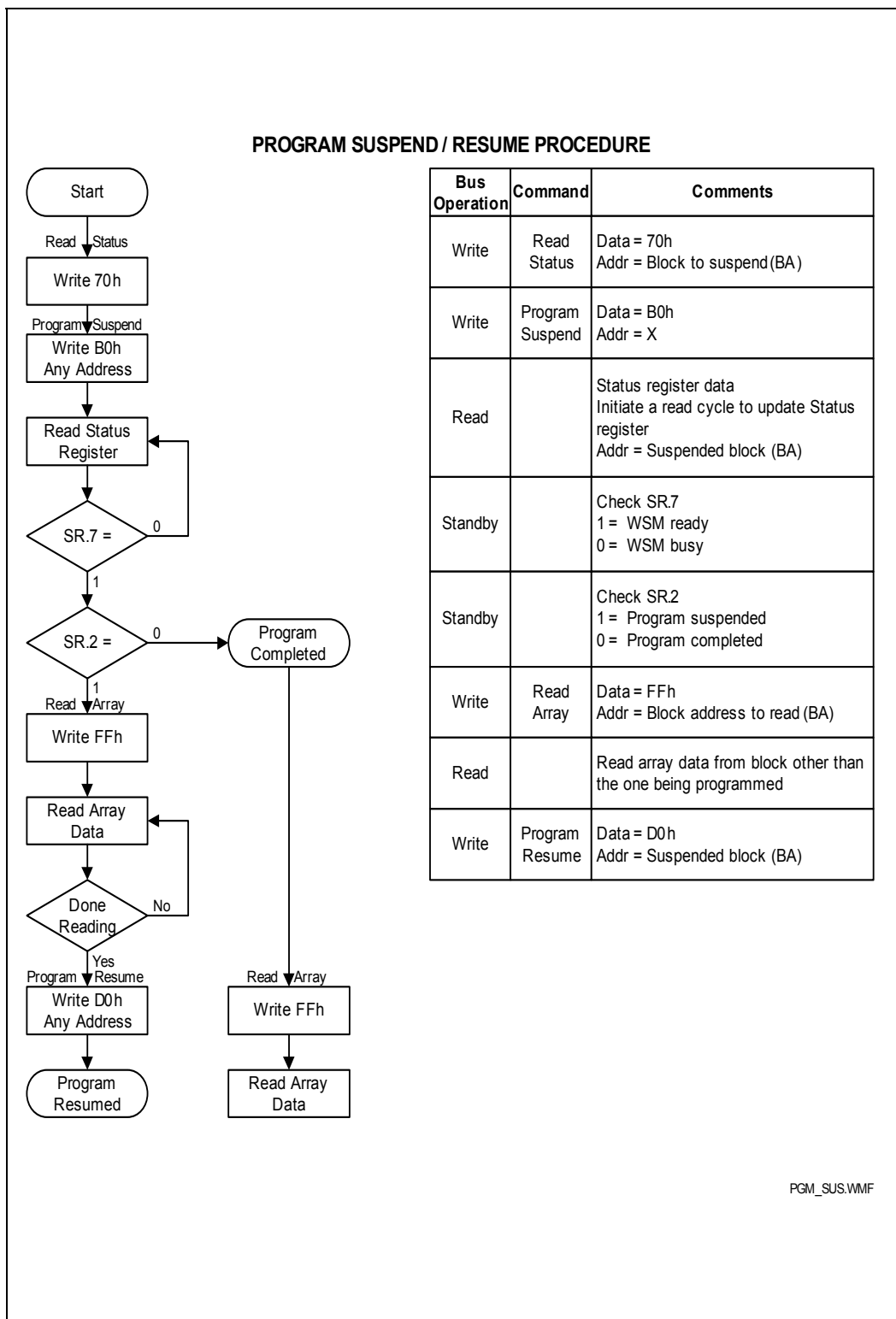
Figure 40. Program Suspend/Resume Flowchart
