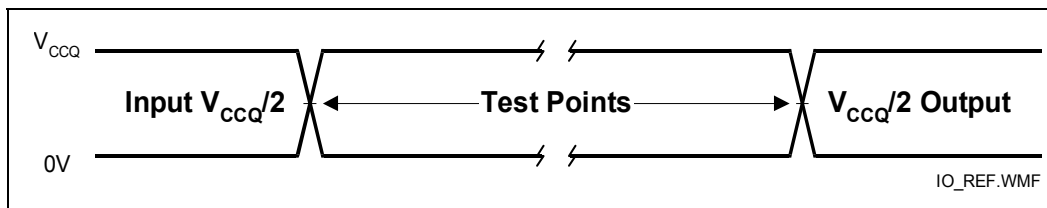
Figure 12. AC Input/Output Reference Waveform
