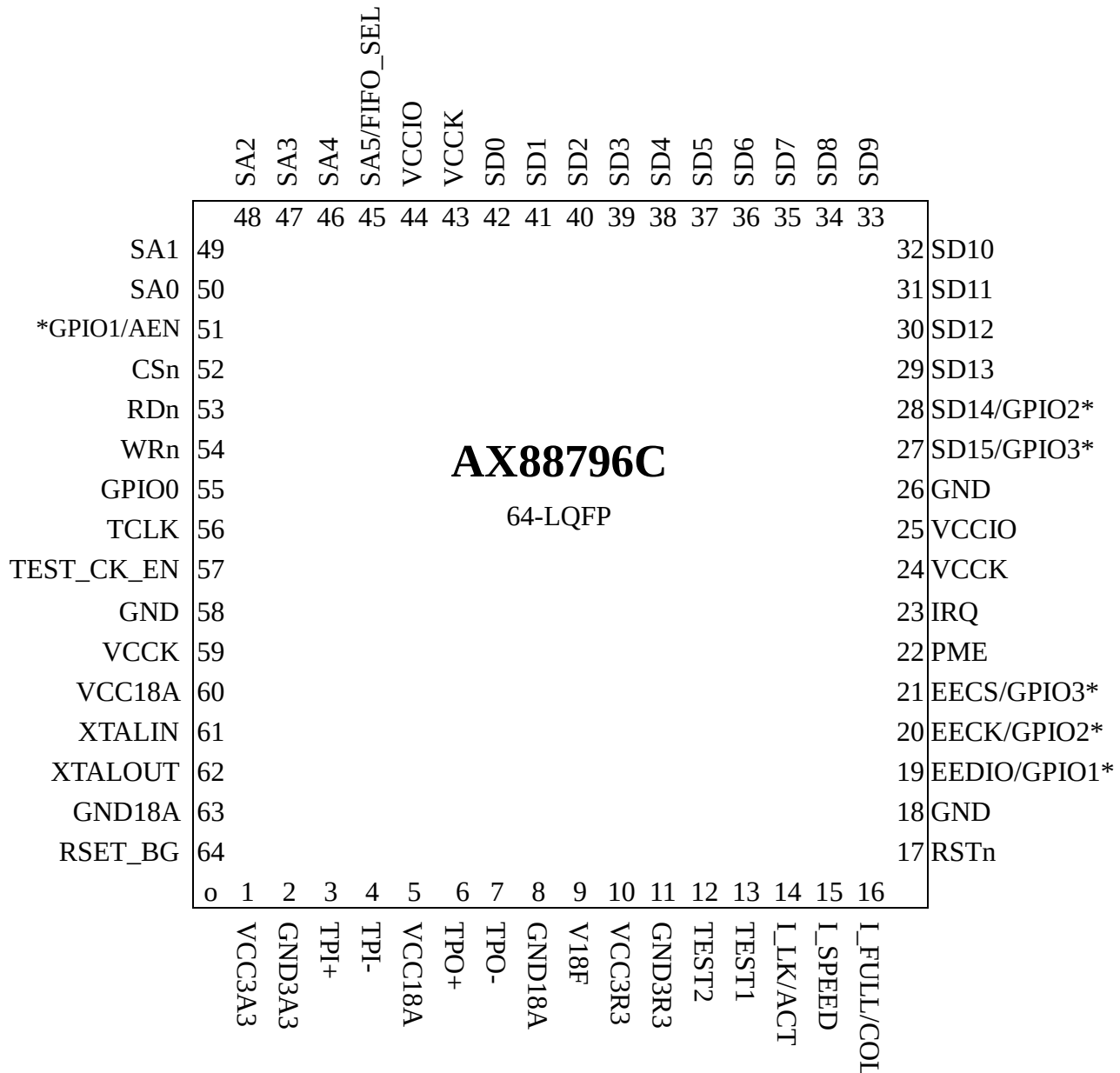
Fig 2 8/16-BIT SRAM-LIKE/RENESAS MODE PIN OUT DIAGRAM
