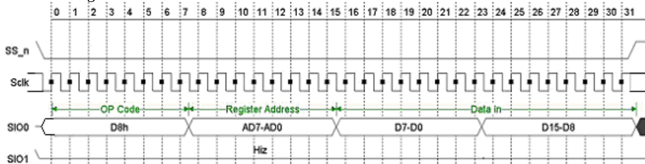
D8h Register Write Command
