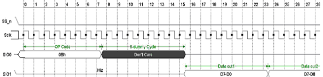
0Bh Fast RXQ Read Command (SPICR SPI_q_compression = 1)
