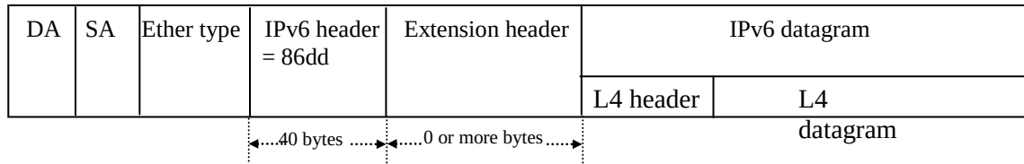
IPv6 packet format
