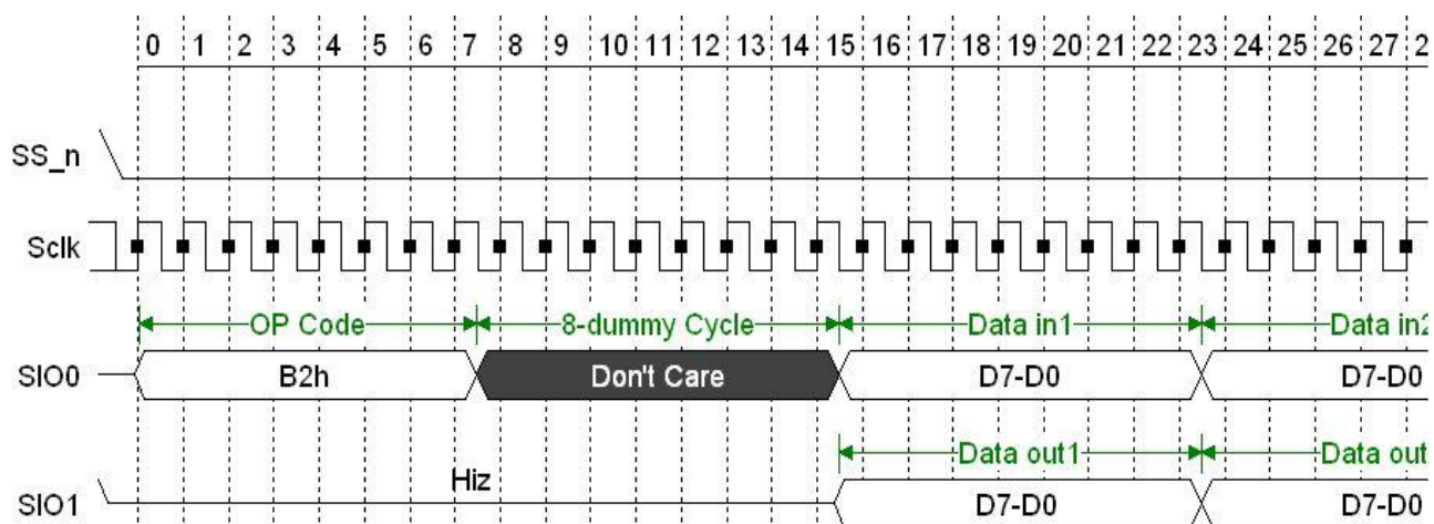
B2h Fast RXQ/TXQ Write Command (SPICR SPI_q_compression =1)
