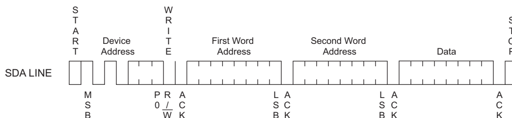
Figure 9-1. Byte Write
