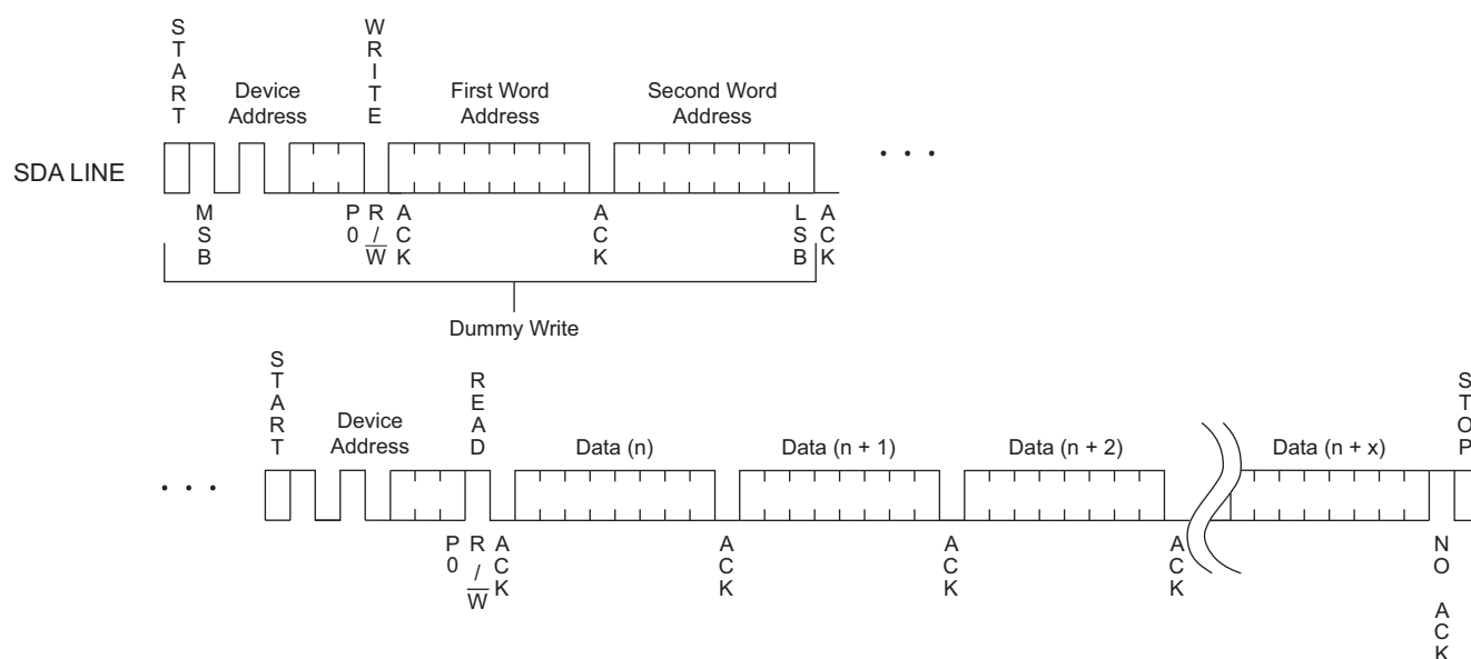
Figure 9-5. Sequential Read
