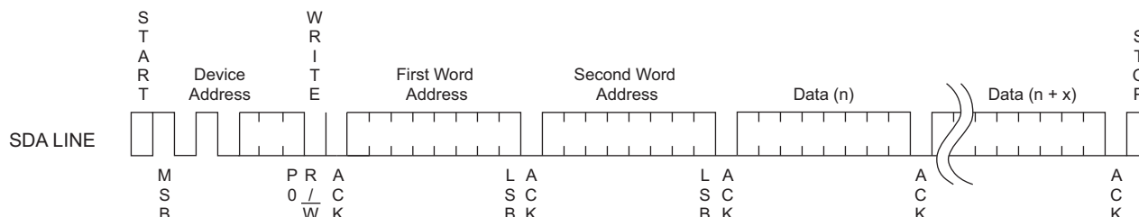
Figure 9-2. Page Write
