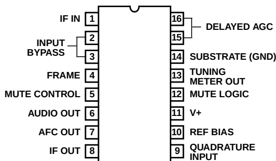
CA3189 (PDIP) TOP VIEW
