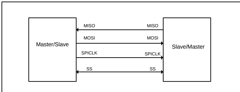
SPI dual device configurarion, where either can be a master or a slave
