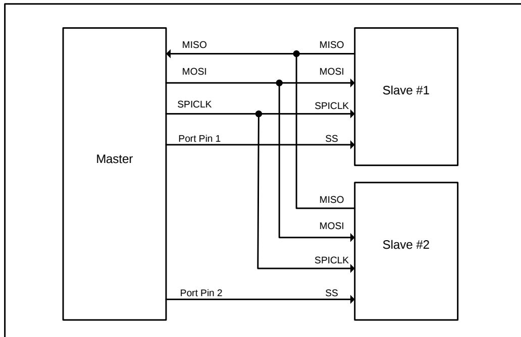
SPI single master multiple slaves configurartion
