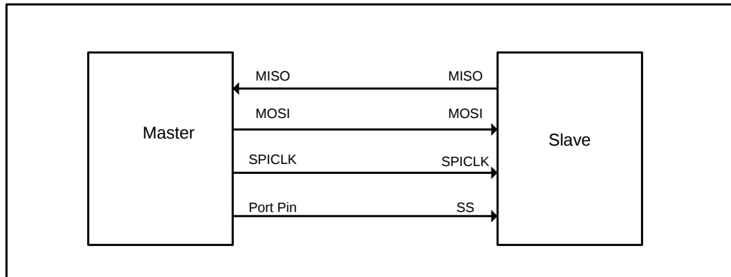
SPI single master single slave configurartion
