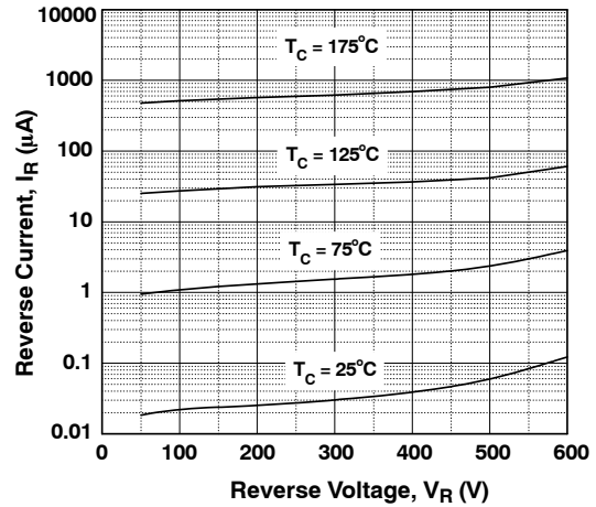
Figure 22. Reverse Current
