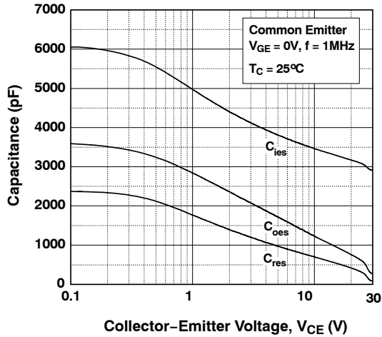
Figure 9. Capacitance Characteristics
