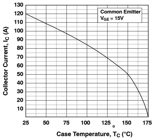
Figure 19. Current Derating
