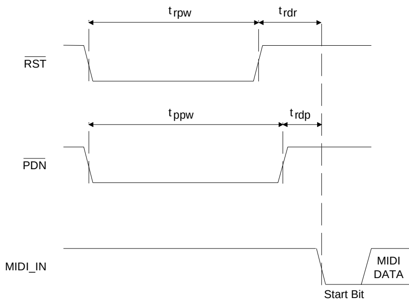
RST/PDN Timing
