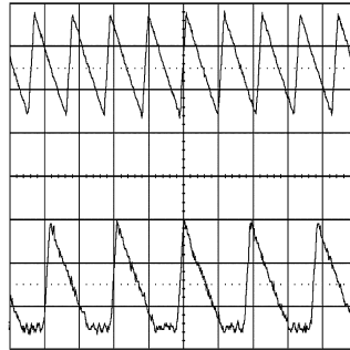
Figure 25. CCM and DCM Operating Modes
