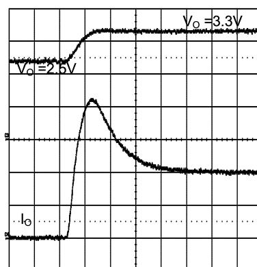
Figure 27. Pre-Biased Startup
