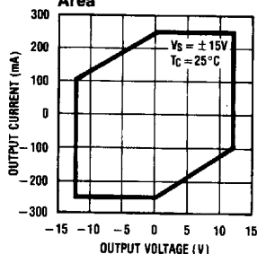
LH0063 DC Safe Operating Area
