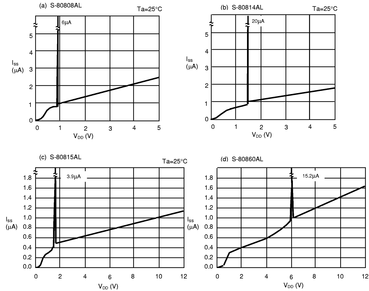
(3) Current consumption ( I_{SS} ) - Input voltage ( V_{DD} )
