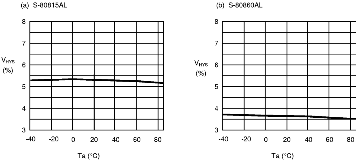
(2) Hysteresis voltage width ( V_{HYS} ) - Temperature ( T_a )
