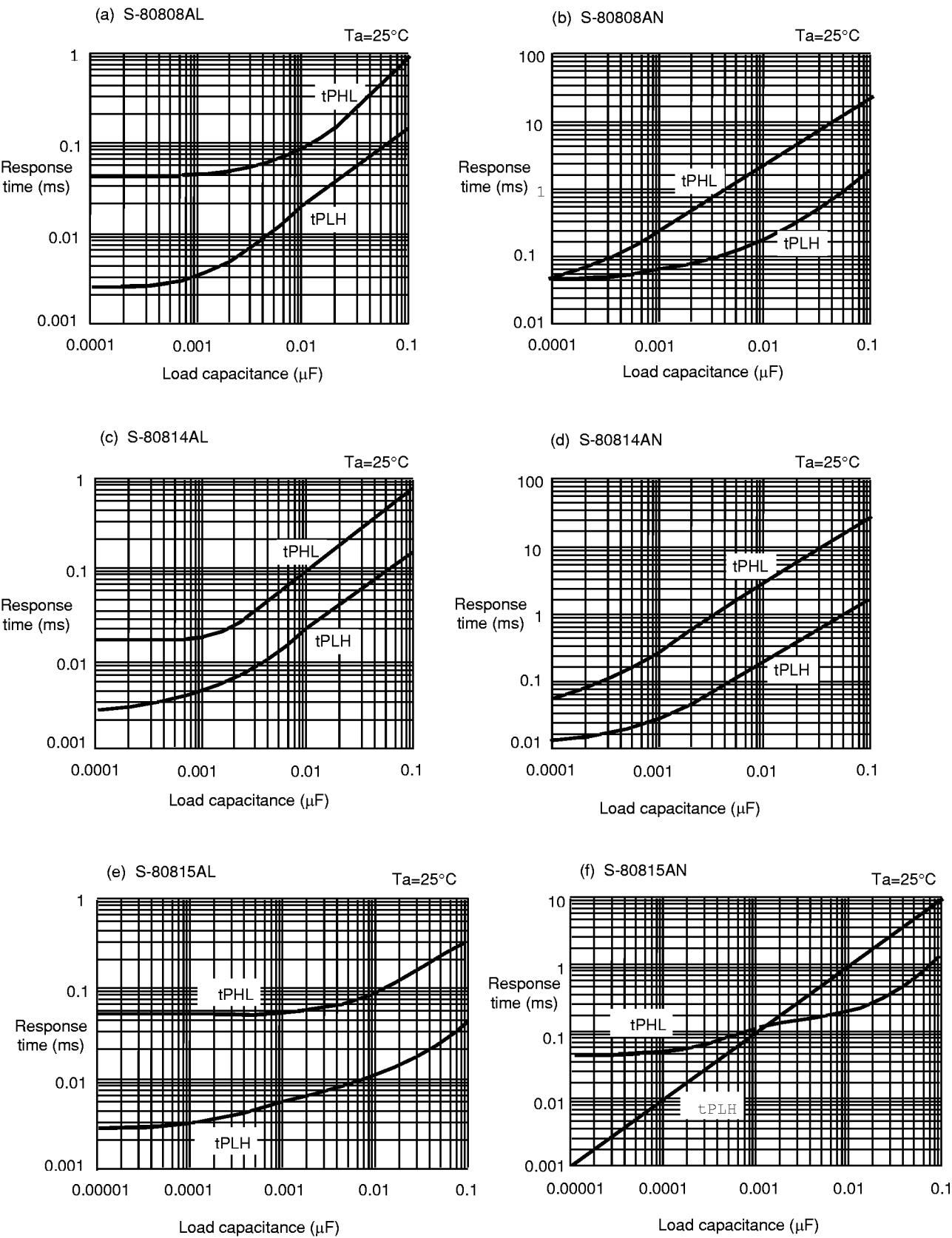
(10) Dynamic response
